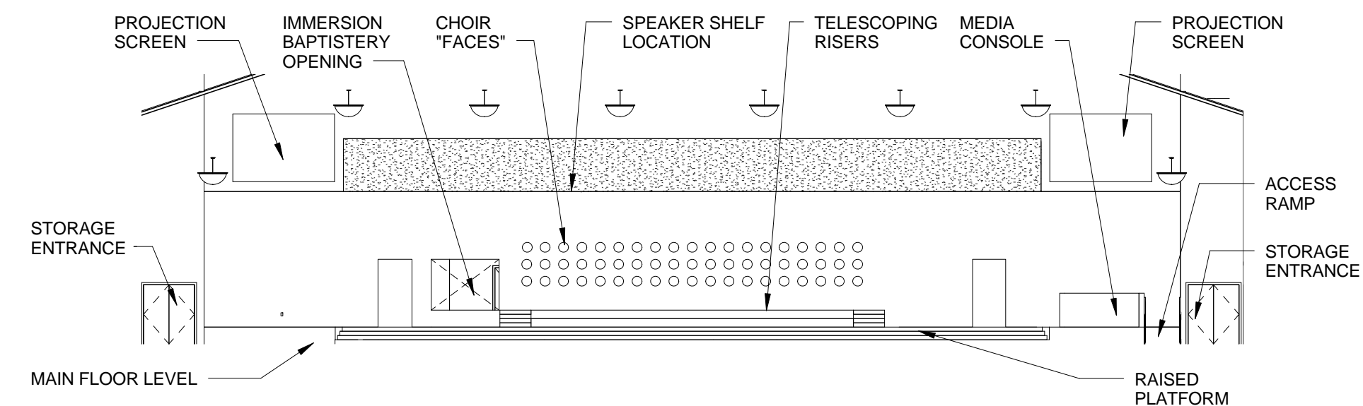
1 INTERIOR ELEVATION A-300 1/16" = 1'-0"
