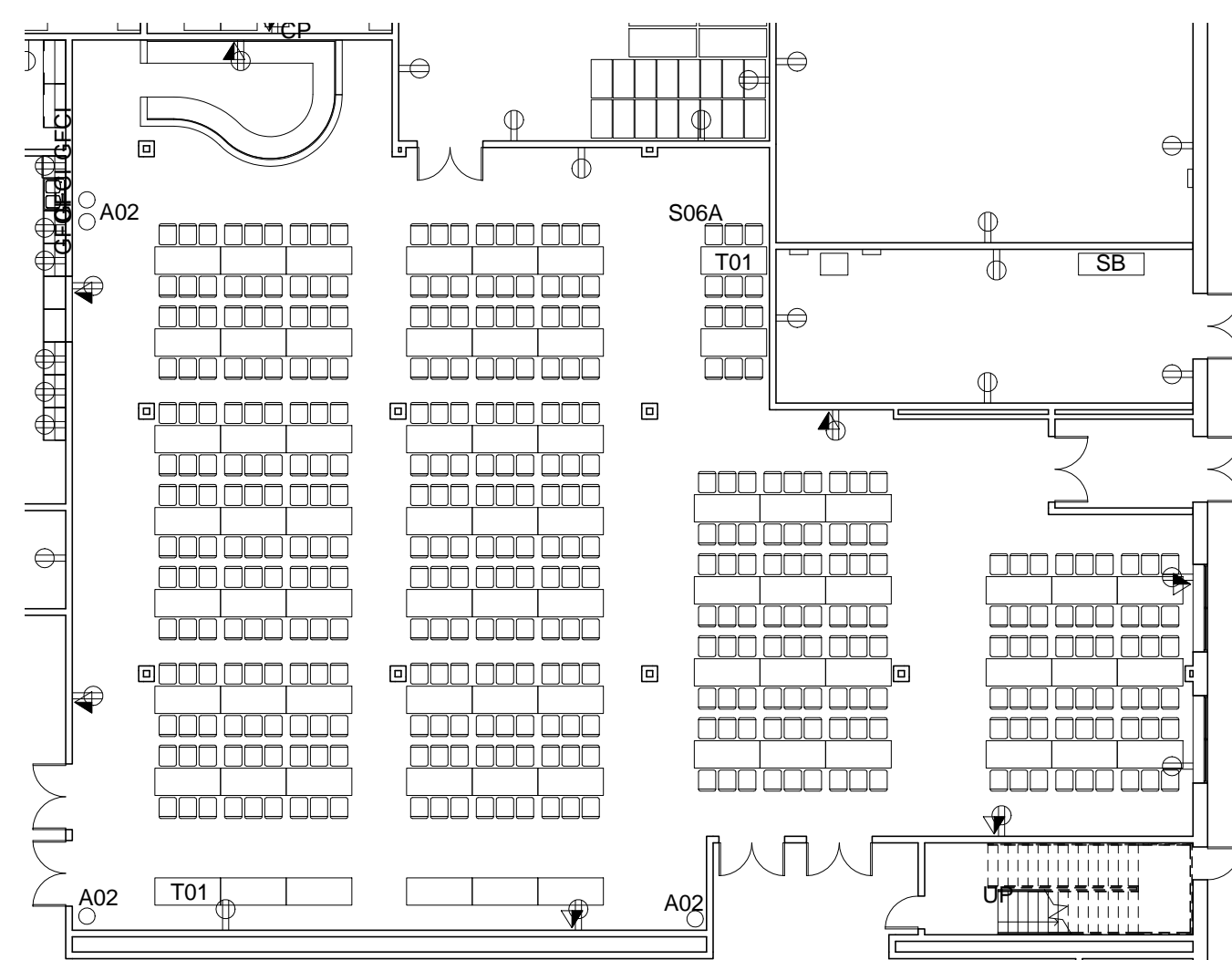
1 ACTIVITY CENTER ALTERNATE LAYOUT I-111 1/16" = 1'-0"
