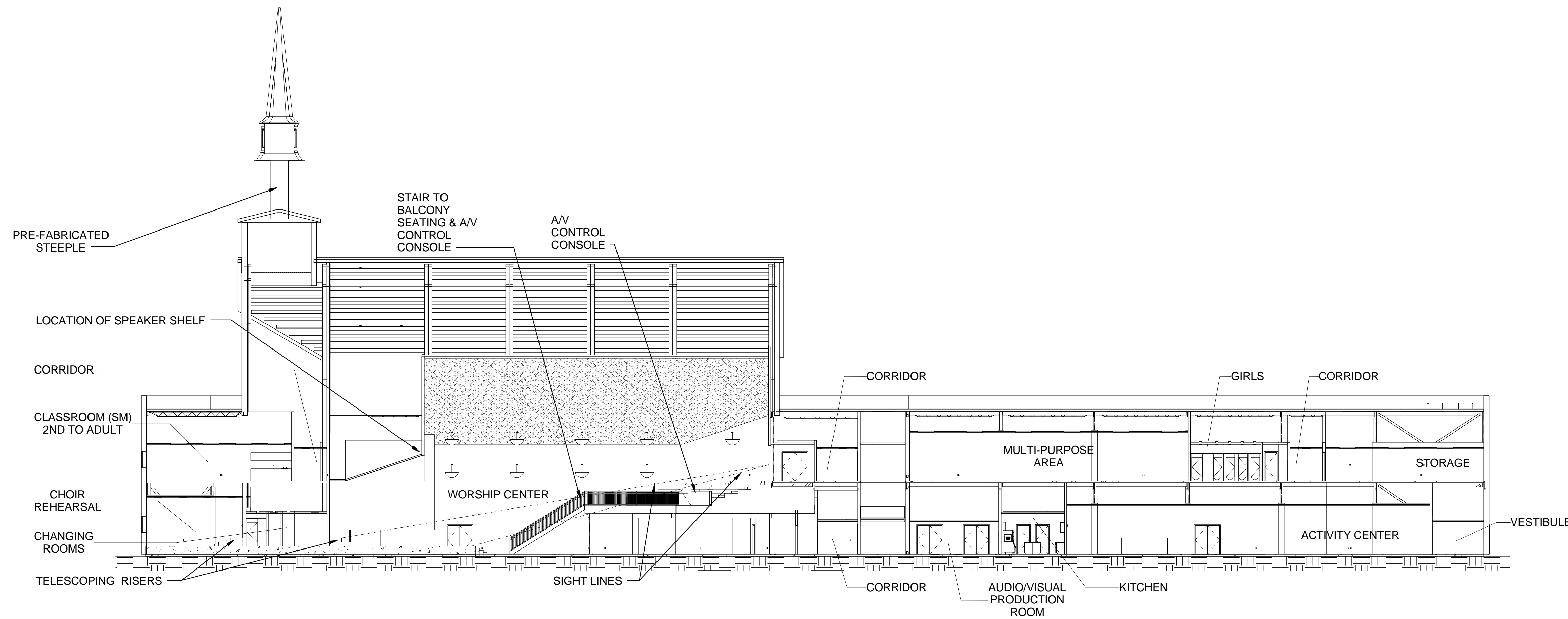
2 BUILDING SECTION A-300 1/16" = 1'-0"
